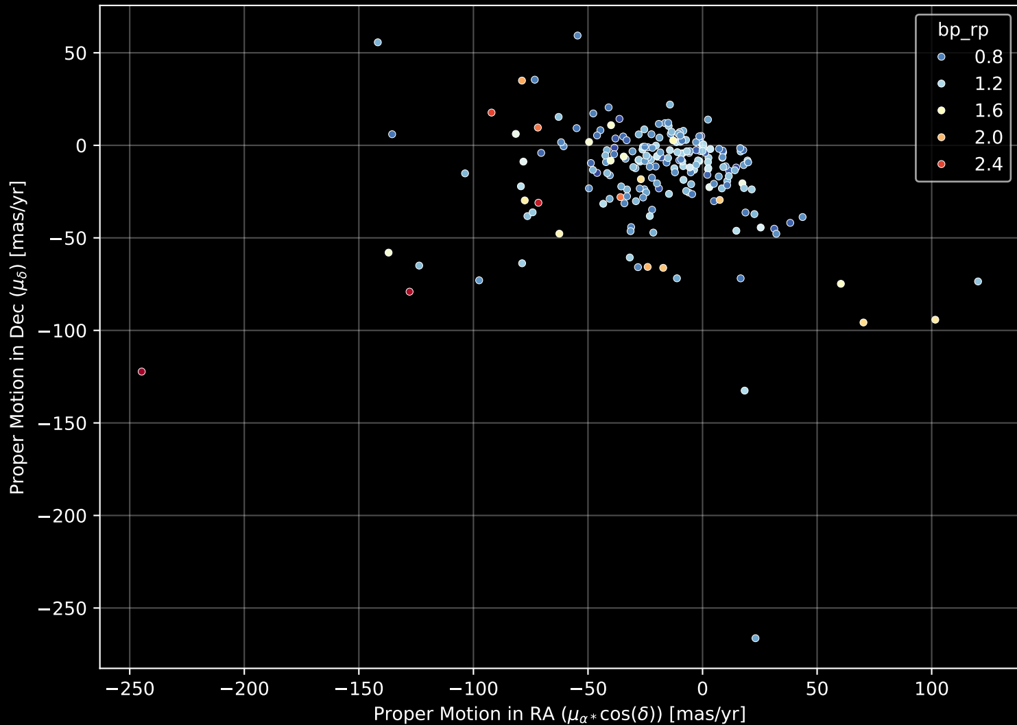
APOGEE DR17 Field: [INTCL_N4147_MGA] Proper Motion Diagram (n= 209)
