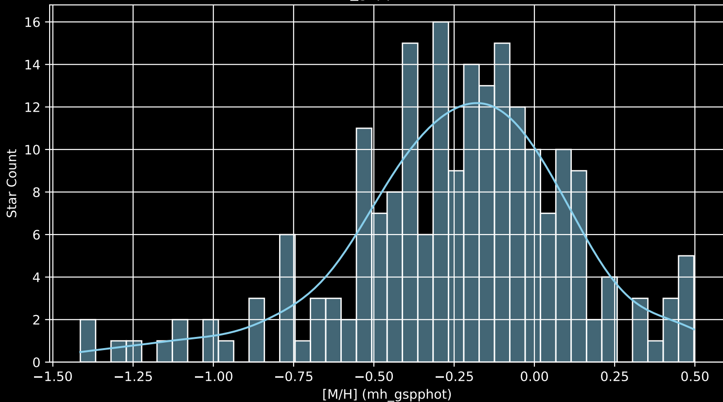
APOGEE DR17 Field: [INTCL_N4147_MGA [M/H] (mh_gspphot) (n= 208)
