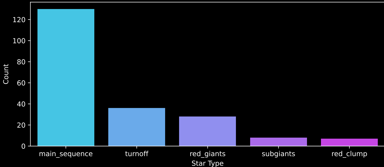
APOGEE DR17 Field: [INTCL_N4147_MGA] Count plot of Star Type
