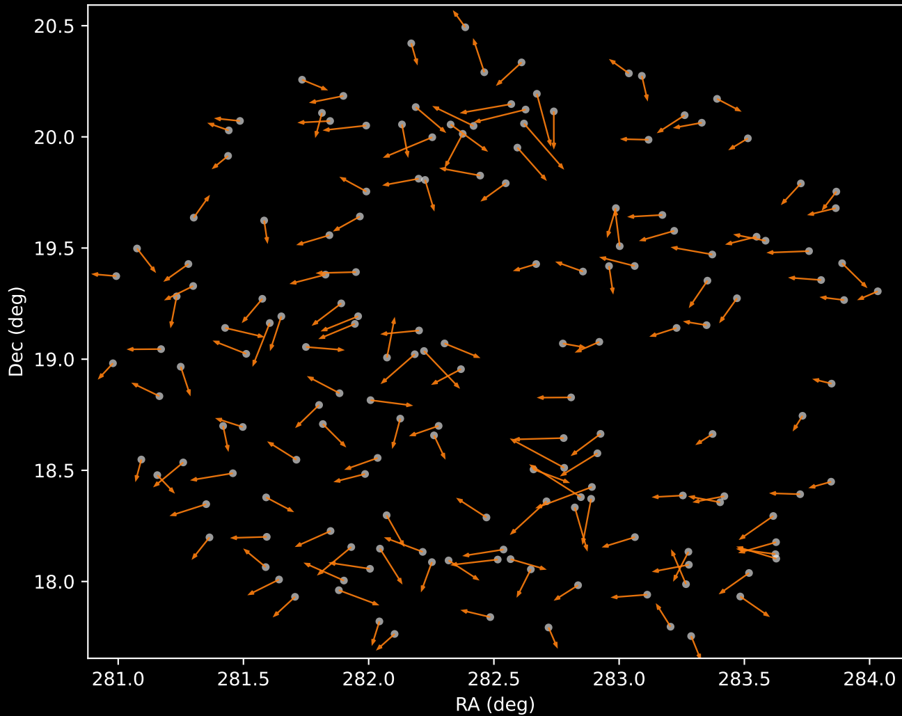
APOGEE DR17 Cluster 2 Proper Motion Vectors (n=166)
