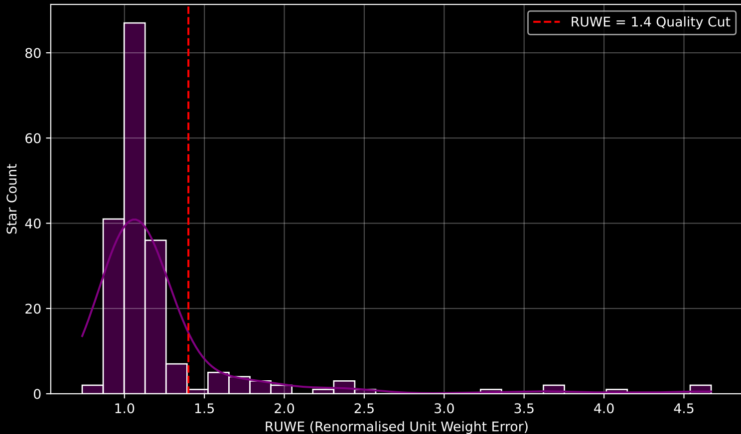
GAPOGEE DR17 Field [INTCL_N4147_MGA] RUWE Distribution (n= 199)
