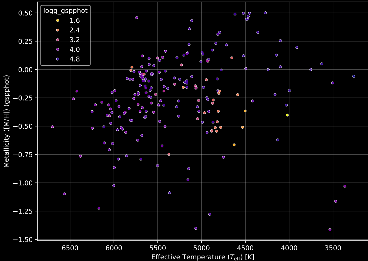
APOGEE DR17 Field: [INTCL_N4147_MGA] Stellar Population Parameters (n= 209)
