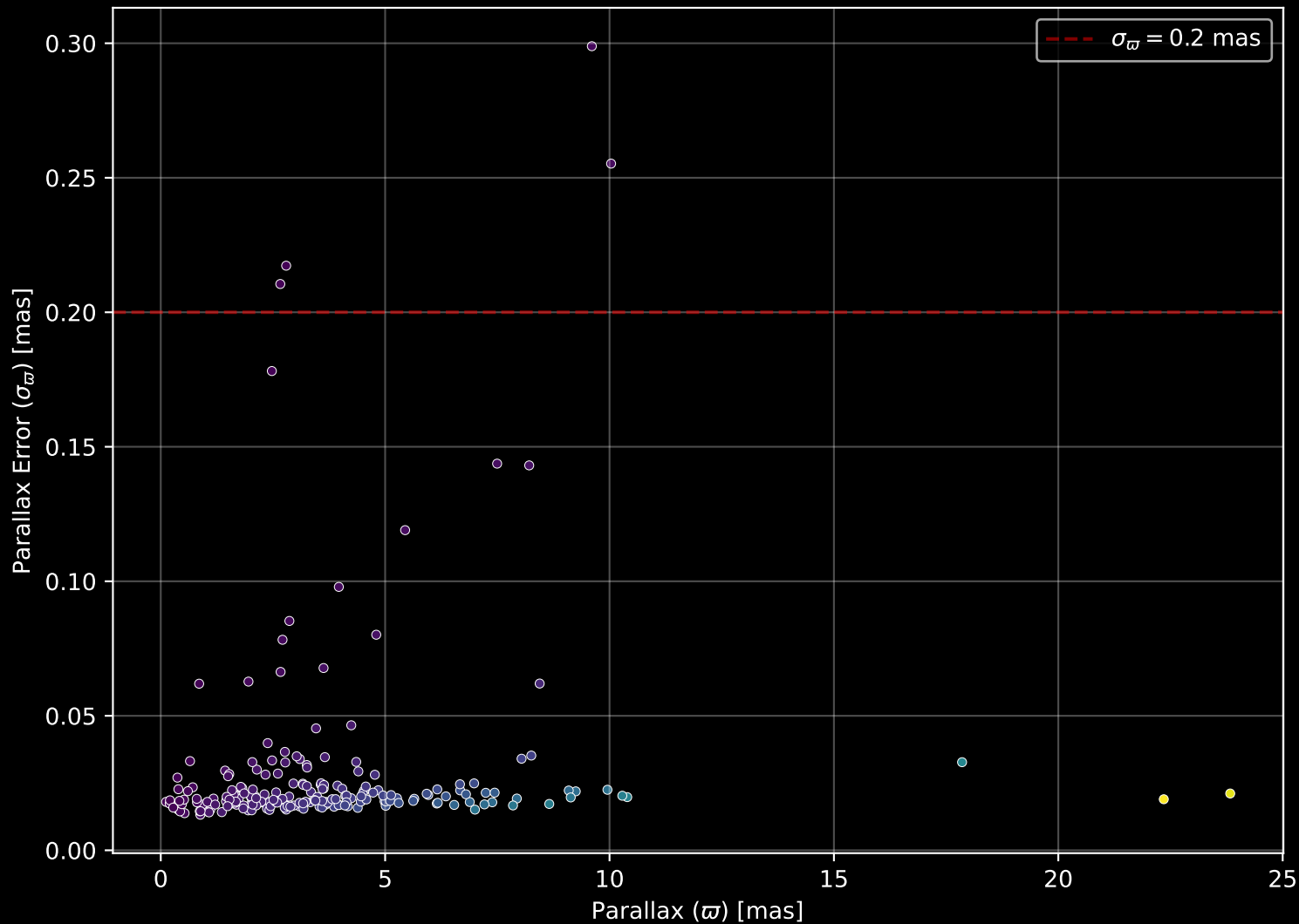
APOGEE DR17 Field: [INTCL_N4147_MGA] Parallax Quality (n= 209)
